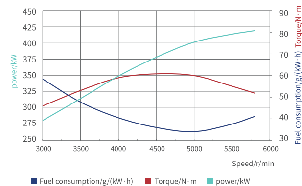
External Characteristic Curve
