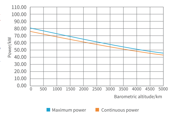
Altitude Characteristic Curve
